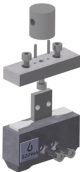
ASTM D 412 Testing Fixture - Assembly
