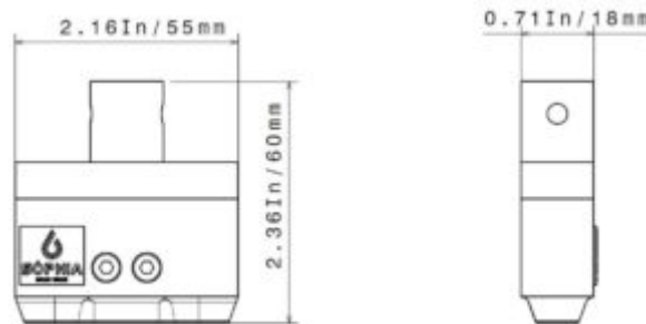
ASTM D 412 Testing Fixture - Drawing
