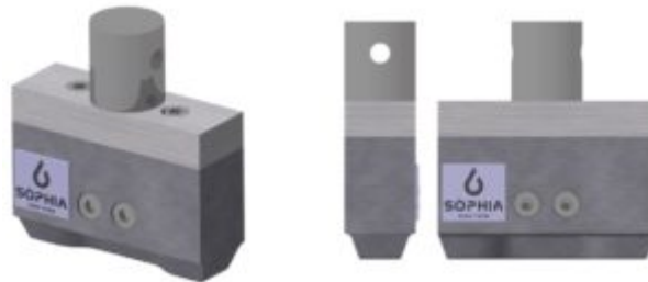
ASTM D412 Testing Fixture
